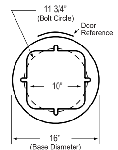
CAV 130 non-illuminated
