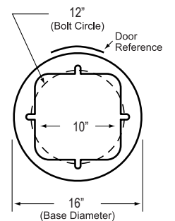
Acorn Finial Ball Top CAV 412 non-illuminated
