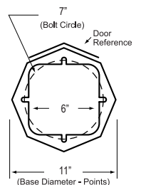
Acorn Finial Ball Top CAV 780 non-illuminated
